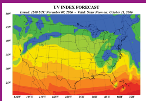
Screenshot of the UV Index Forecast, prepared daily by the National Weather Service.
