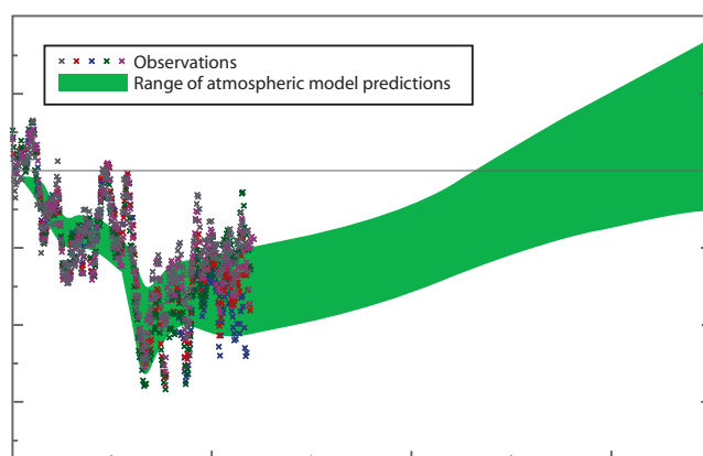
Global Ozone Depletion and Recovery
